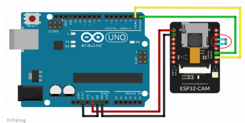
Figure 2: System wiring
